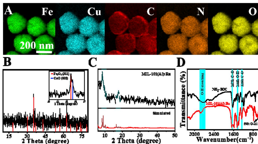
Fig. 2. (A) TEM mapping images of Fe, O, Cu, C, N elements in Fe 3 O 4 @PDA-Cu x O. (B) XRD pattern of Fe 3 O 4 @PDA-Cu x O. (C) XRD pattern of MIL-101(Al):Ru. (D) Infrared spectra of NH 2 -BDC and MIL-101(Al):Ru.
