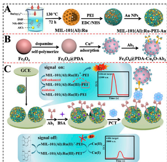
Scheme 1. Schematic diagrams for (A) the synthesis steps of MIL-101(Al):Ru-PEI-Au, (B) the synthesis steps of Fe 3 O 4 @PDA-Cu x O-Ab 2 , (C) the fabrication process of PCT sensor and the possible luminescence mechanism.
