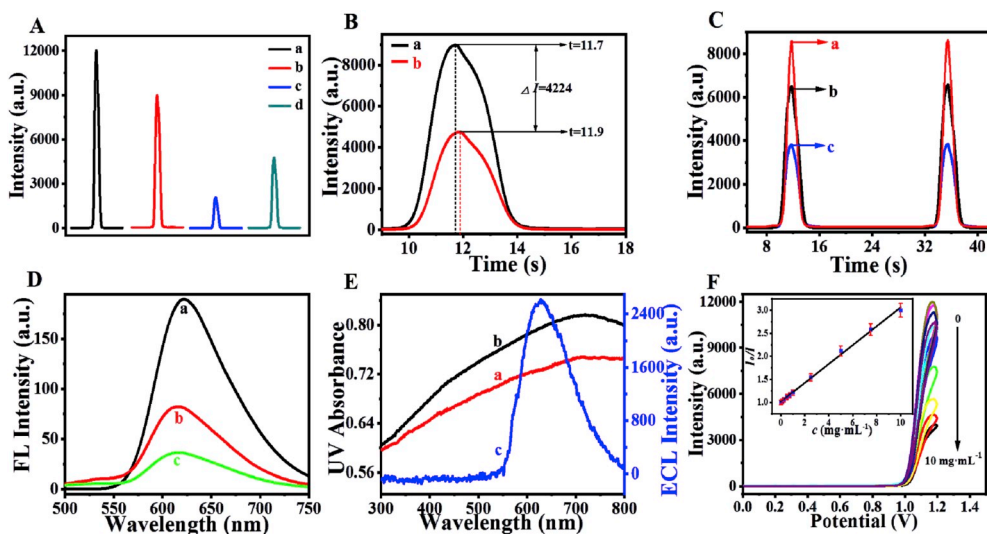
ECL spectra of MIL-101(Al):Ru. (F) ECL intensities of MIL-101(Al):Ru-PEI-Au in the presence of 0, 0.1, 0.25, 0.5, 0.75, 1, 2.5, 5, 7.5, 10 mg mL -1 of Fe 3 O 4 @PDA-Cu x O. Inset: Stern-Volmer quenching intensity plot of MIL-101(Al):Ru-PEI-Au by Fe 3 O 4 @PDA-Cu x O in 10 mL of PBS (pH 7.4).
