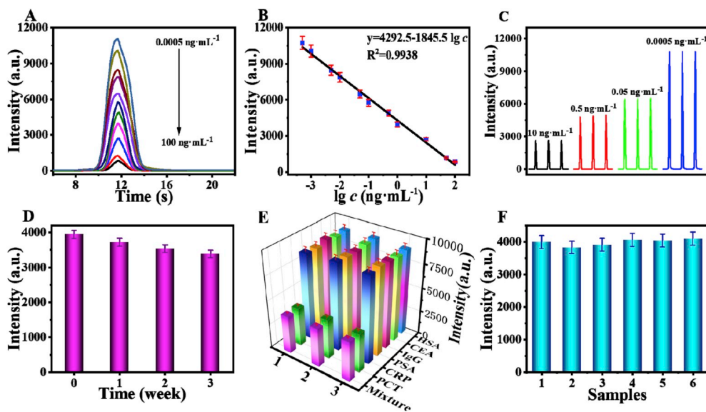
Fig. 5. (A) ECL intensity-time curves of the immunosensor in the presence of different concentrations of PCT: 0.0005, 0.001, 0.005, 0.01, 0.05, 0.1, 0.5, 1, 10, 50, 100 ng mL -1 . (B) Calibration plots of the immunosensor. (C) stability of the immunosensor to various concentrations of PCT. (D) Long-term storage stability of the sensor incubated with 1 ng mL -1 of PCT. (E) Selectivity of the immunosensor: 10 ng mL -1 of HSA, CEA, IgG, PSA, CRP and 1 ng mL -1 of PCT with their mixture. (F) Reproducibility of the immunosensor incubated with 1 ng mL -1 of PCT.
