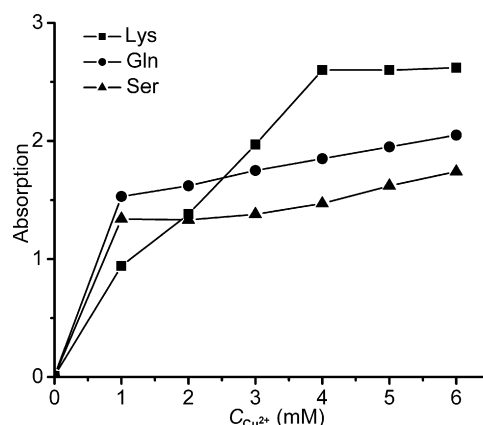
Fig. 3. Effect of cupric cation concentration on UV signals of Lys, Gln and Ser at 232 nm.
