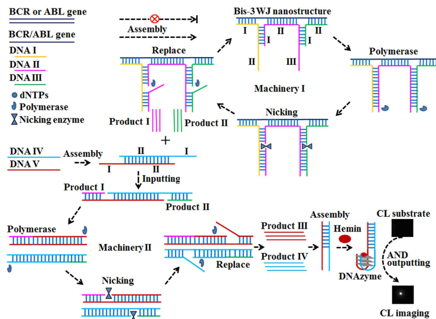
Figure 1. Schematic illustration of the imaging method for BCR/ABL fusion gene detection base on bis-3WJ nanostructure and DNA machineries.
