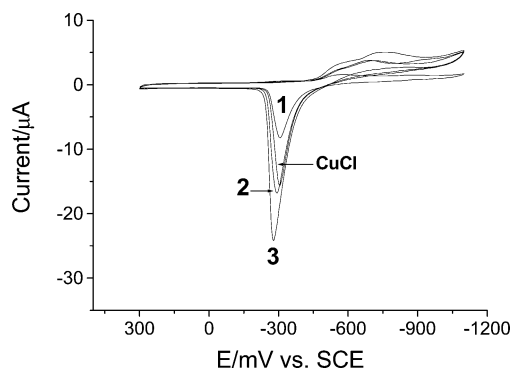
Figure 4. Cyclic voltammograms of 0.1 M Bu 4 NClO 4 acetonitrile solutions containing 1.0 mM CuCl, [(2-H 2 PYA) 2 Cu 2 Cl 4 ] n ( 1 ), [(3-H 2 PYA) 2 Cu 2 Cl 4 ] n ( 2 ), and [(4-H 2 PYA) 2 Cu 2 Cl 4 ] n ( 3 ) at 100 mV/s at a platinum disk working electrode.
