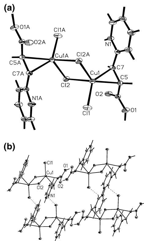
Figure 1. (a) Dimeric molecular structural representation of 1 (30% ellipsoid probability). Typical bond distances (Å) and angles (deg): Cu(1)—Cl(1) 2.2443(6), Cu(1)—Cl(2) 2.3205(6), Cu(1)—Cl(2A) 2.4870(6), Cu(1)—C(5) 2.066(2), Cu(1)—C(7) 2.092(2), C(5)—C(7) 1.375(3); C(5)—Cu(1)—C(7) 38.62(8), C(5)—Cu(1)—Cl(1) 103.62(6), C(7)—Cu(1)—Cl(2A) 105.47(6), Cl(1)—Cu(1)—Cl(2) 104.23(2), Cl(1)—Cu(1)—Cl(2A) 104.58(2), Cl(2)—Cu(1)—Cl(2A) 97.02(2), Cu(1)—Cl(2)—Cu(1A) 82.98(2). (b) 3-D network representation of 1 through H-bonds in which a carboxylic acid dimer was yielded via H-bonds.
