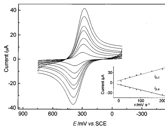
Fig. 2 Cyclic voltammograms of Os-(PVP) 10 /Nafion modified electrode in 0.1 M PBS (pH 7.0) at 200, 150, 100, 80, 50, 30 and 10 \text{mV s}^{-1} (from highest to lowest peak currents). Inset: plots of peak current versus scan rate.
