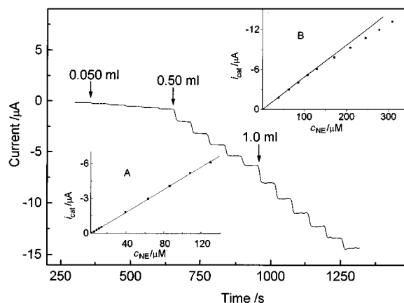
Fig. 5 Chronoamperometric response currents of NE at \text{Os}-(\text{PVP})_{10}/\text{Nafion} modified electrode in 25.0 ml of pH 7.0 PBS after successive addition of 50 \mu\text{l} (five times), 0.50 ml (five times) and 1.0 ml (five times) of 1.3 mM NE at an applied potential of +0.5 V. Inset: plots of catalytic current versus NE concentration.
