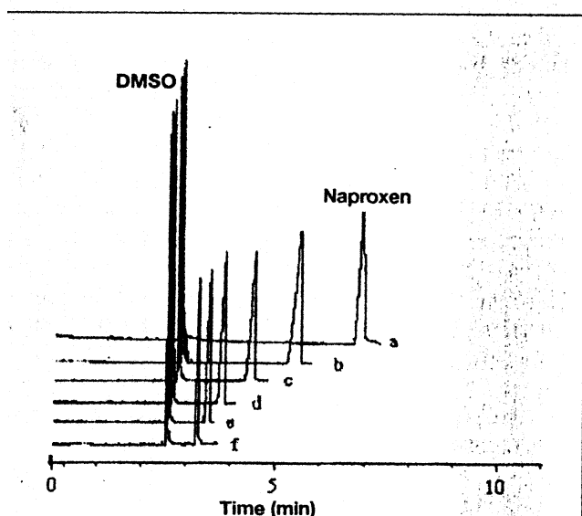
Figure 1. Migration time of naproxen as a function of \beta -CD concentration in the running buffer: injection of naproxen, 50 mbar, 3 s; voltage, 15kV; temperature, 25°C; UV detection, 214 nm; and buffer, 20mM (pH 7.0) PBS including 0, 0.5, 1.0, 2.5, 5.0, and 7.5mM \beta -CD for a–f.
