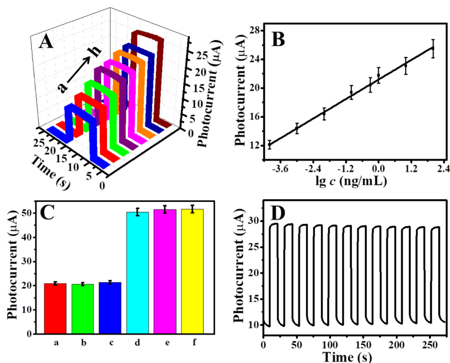
Fig. 4. (A) Photocurrent response curve and (B) the logarithmic calibration curve of the PEC immunosensor for detection of different concentrations of NT-Pro BNP: (a) 0.0001, (b) 0.001, (c) 0.01, (d) 0.1, (e) 0.5, (f) 1, (g) 10, (h) 100 (Units: ng/mL). (C) Selectivity detection of the prepared PEC immunosensor for NT-Pro BNP. (a) 1.0 ng/mL NT-pro BNP + 100 ng/mL CEA; (b) 1.0 ng/mL NT-pro BNP + 100 ng/mL PSA; (c) 1.0 ng/mL NT-pro BNP + 100 ng/mL insulin; (d) 100 ng/mL CEA; (e) 100 ng/mL PSA; (f) 100 ng/mL insulin; (D) Stability evaluation of the PEC immunosensor under several on/off irradiation cycles, c_{\text{NT-Pro BNP}} = 1.0 \text{ ng/mL} . The applied potential was 0 V.
