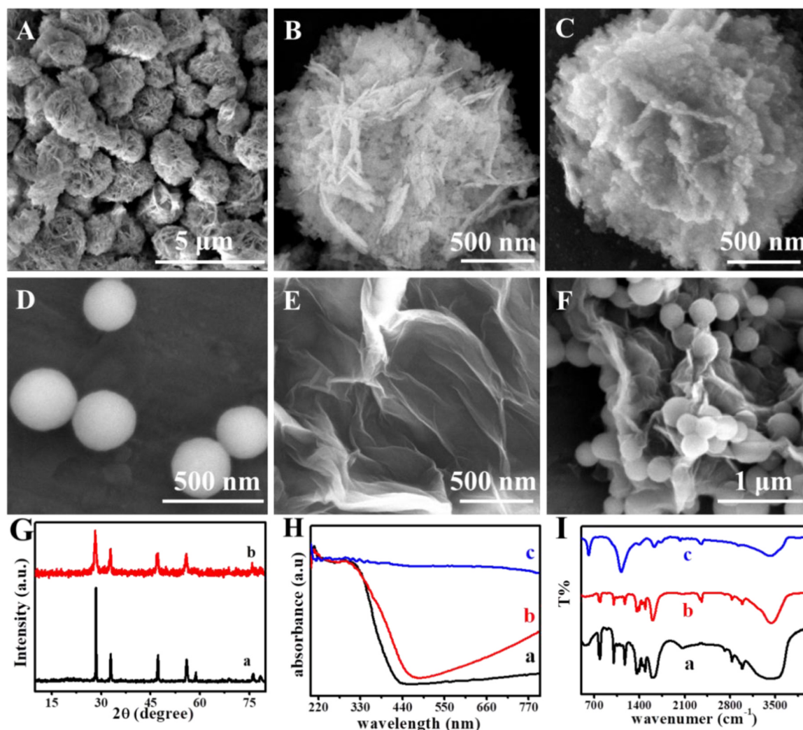
Fig. 1. SEM images of (A and B) F-Bi 2 WO 6 , (C) F-Bi 2 WO 6 /Ag 2 S, (D) PDA, (E) GO and (F) GO/PDA, respectively; (G) XRD spectrum of (a) F-Bi 2 WO 6 , (b) F-Bi 2 WO 6 /Ag 2 S; (H) UV-vis diffuse reflectance spectra of (a) F-Bi 2 WO 6 , (b) F-Bi 2 WO 6 -TGA and (c) F-Bi 2 WO 6 /Ag 2 S; (I) FTIR spectrum of (a) GO/PDA, (b) PDA, (c) GO.
