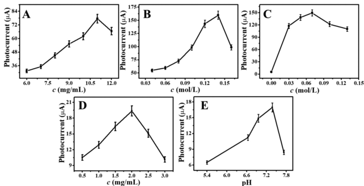
Fig. 3. Optimization of experimental conditions: (A) F-Bi 2 WO 6 concentration, (B) AgNO 3 concentration, (C) AA concentration in the PBS on the photocurrent response of ITO/F-Bi 2 WO 6 /Ag 2 S electrodes, (D) GO/PDA composite concentration on the photocurrent response of ITO/F-Bi 2 WO 6 /Ag 2 S/Ab 1 /BSA/NT-Pro BNP/GO/PDA-Ab 2 electrodes (E) the pH value of PBS. The applied potential was 0 V. For all studies, error bars = SD ( n = 5 ).
