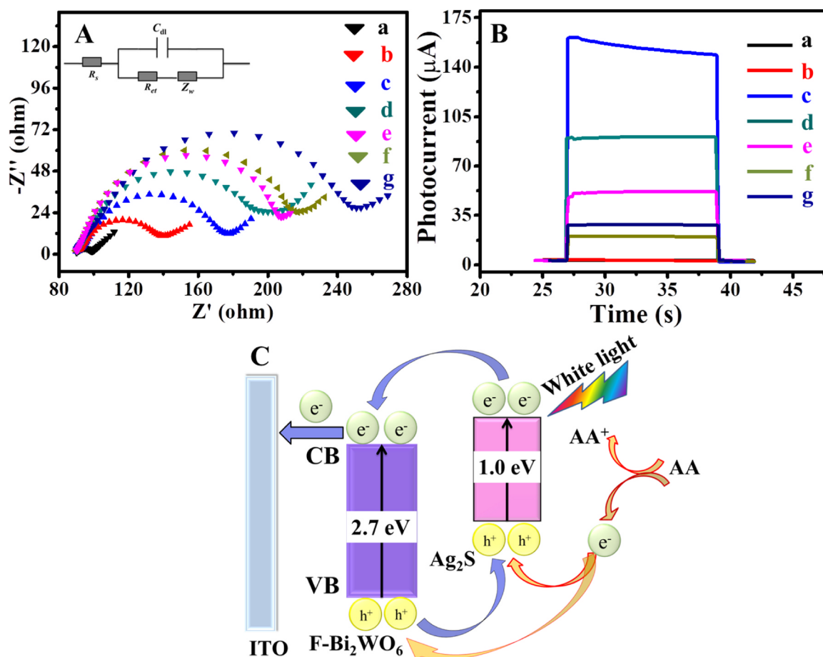
Fig. 2. (A) EIS Nyquist plots and (B) time-based photocurrent response curves of (a) ITO electrode, (b) after F-Bi 2 WO 6 deposition, (c) after Ag 2 S sensitization, (d) after Ab 1 incubation, (e) after BSA blocking, (f) after 1.0 ng/mL NT-Pro BNP incubation; (g) after GO/PDA-Ab 2 incubation. (C) The illustration of electron-transfer mechanism of PEC immunosensor based on F-Bi 2 WO 6 /Ag 2 S in PBS solution containing AA. The inset in (A) is Randles equivalent circuit for EIS. The applied potential was 0 V.
