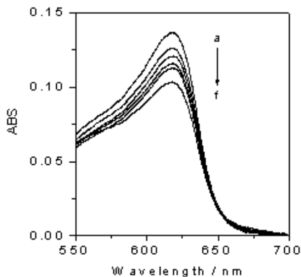
Figure 5. UV spectra of 0.5 mM \text{FcPF}_6 in different dsDNA concentrations of 0, 20, 40, 60, 80 and 100 \mu\text{g ml}^{-1} from (a) to (f).
