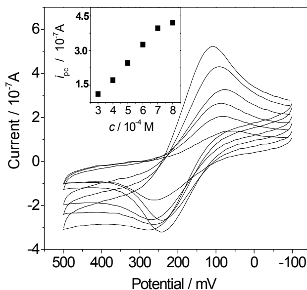
Figure 4. Cyclic voltammograms of 0.3, 0.4, 0.5, 0.6, 0.7 and 0.8 mM FcPF 6 (from internal to external) at ssDNA/SAM/Au at 200 mV s -1 . Inset: plot of i_{pc} vs. concentration of Fc + .
