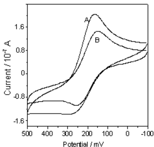
Figure 2. Cyclic voltammograms of 0.4 mM FcPF 6 at bare gold (A) and SAM/Au (B) electrodes at 200 mV s -1 .
