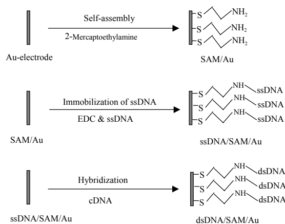
Figure 1. The preparation procedure of DNA sensor.
